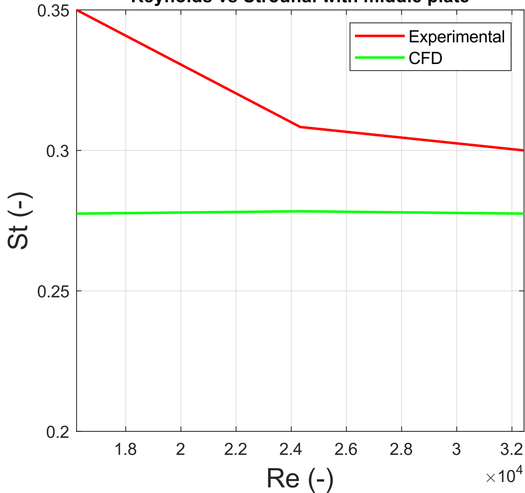
Reynolds vs Strouhal with middle plate
